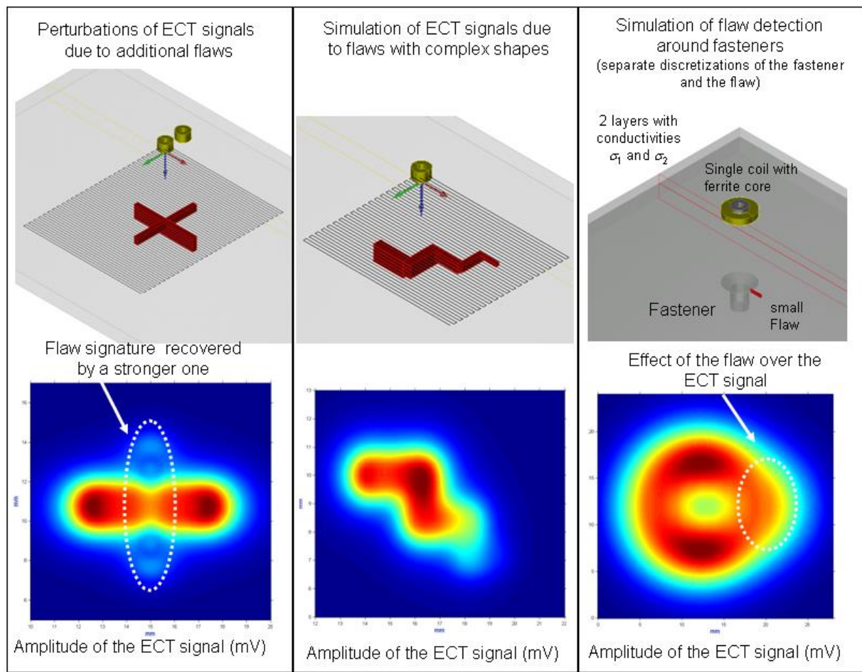
Figure 4 : Three examples of new configurations simulated using multiple flaws. On the left side, modeling of the shading effect of one flaw on one another. In the center: modeling of flaws with complex shapes. On the right side: improvement of interactions calculations between objects like a rivet and a flaw.
