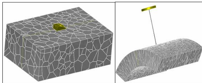
Figure 1: Example of Voronoi diagrams representation for a planar, equiaxed component, and a cylinder with columnar grains
