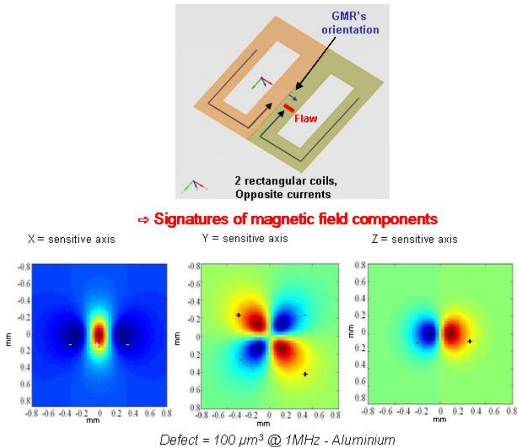
Figure 5: Above: typical probe configuration using a GMR as a receiver. The emitting part consists in two rectangular coils creating a "double D" shape. Below: ECT C-scans obtained for three different orientations of the GMR.
