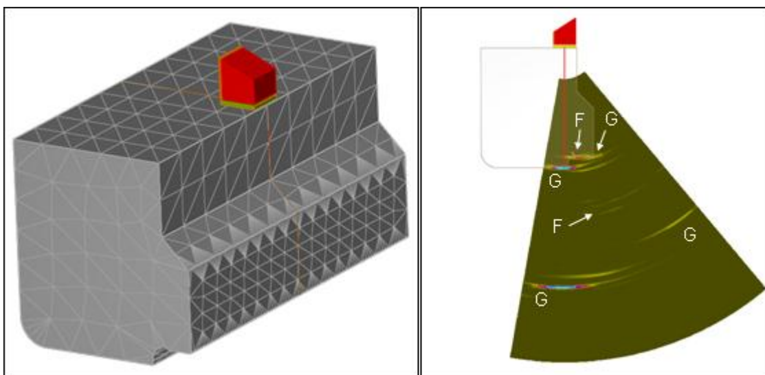
Figure 3: Meshed 3D CAD component (left) and sectorial scan image (right) part.
