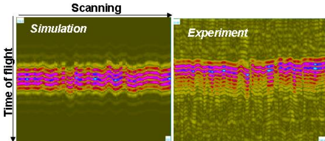
Fig 2: Simulated (left) and measured (right) backwall echo of a CSS cylindrical part.
