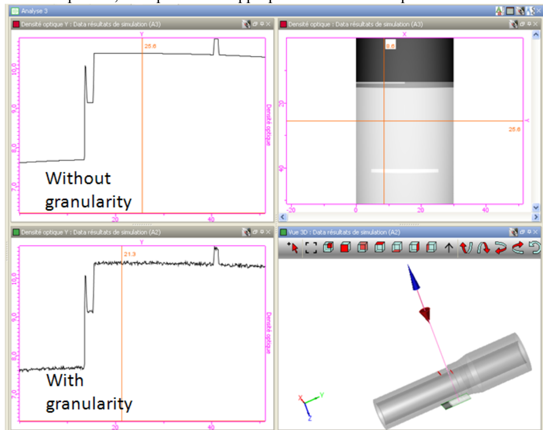
Figure 6: Comparison of two simulations: one taking into accounts the granularity, the other one without granularity
