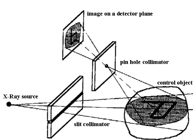
Figure 1. Scanning chart on the basis of the flat detector matrix and pin hole aperture
