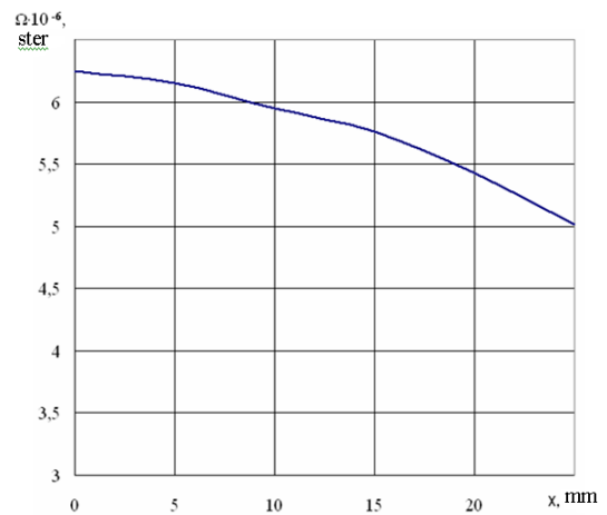
Figure 5. Graph \Omega(x)
