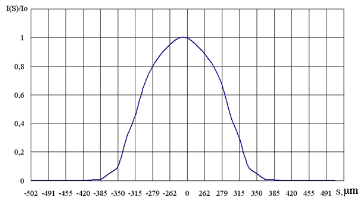
Figure 6. Aperture function of the pin hole with triangle form sponges
