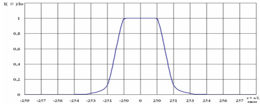
Figure 3. Aperture function of the pin hole system of selection
