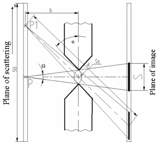
Figure 4. Geometry of change of corporal corner depending on a coordinate x .
