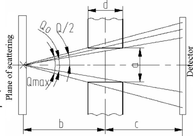
Figure 2. Geometry of the weakening in the walls of pin hole ( a = d = 1\text{mm} , b = c = 50\text{mm} )
