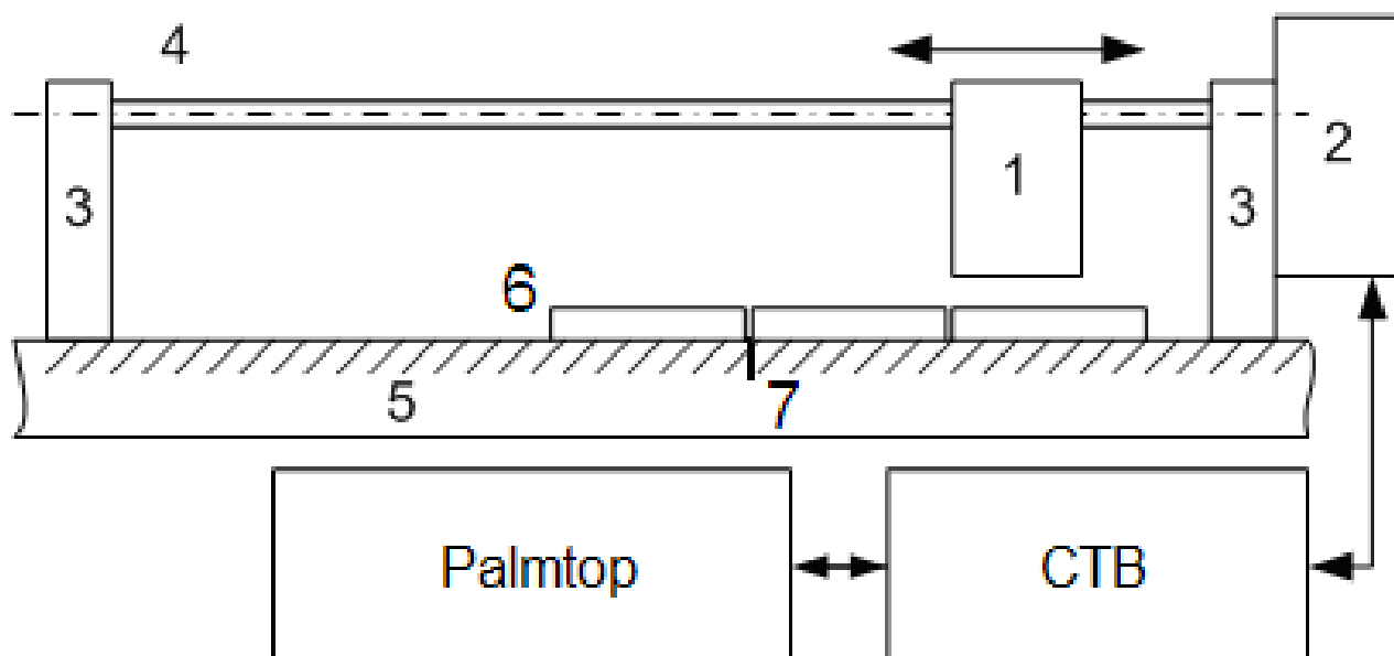
Fig. 1 Basic kinematic scheme of the scanning mechanism
