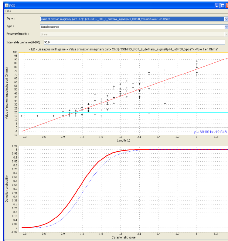
Figure 4: CIVA result panel for Signal Response analysis and corresponding POD
