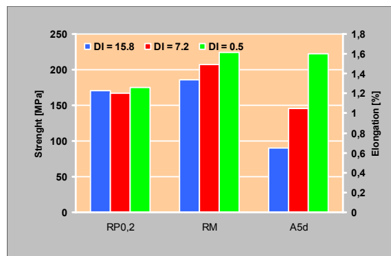
Fig. 5: Mechanical properties
