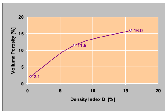
Fig. 4: Density index vs. polume porosity
