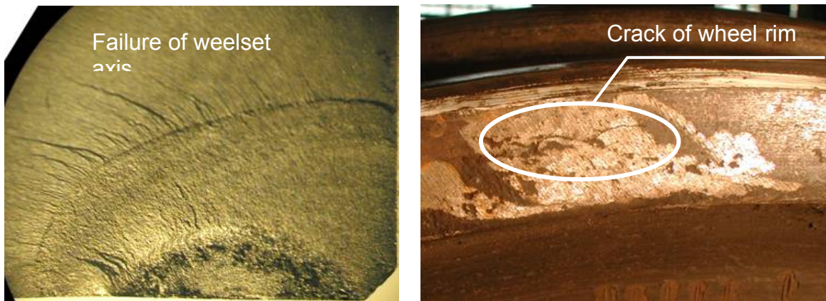
Fig.6. The defects detected in wheelset pairs using AE diagnostics
