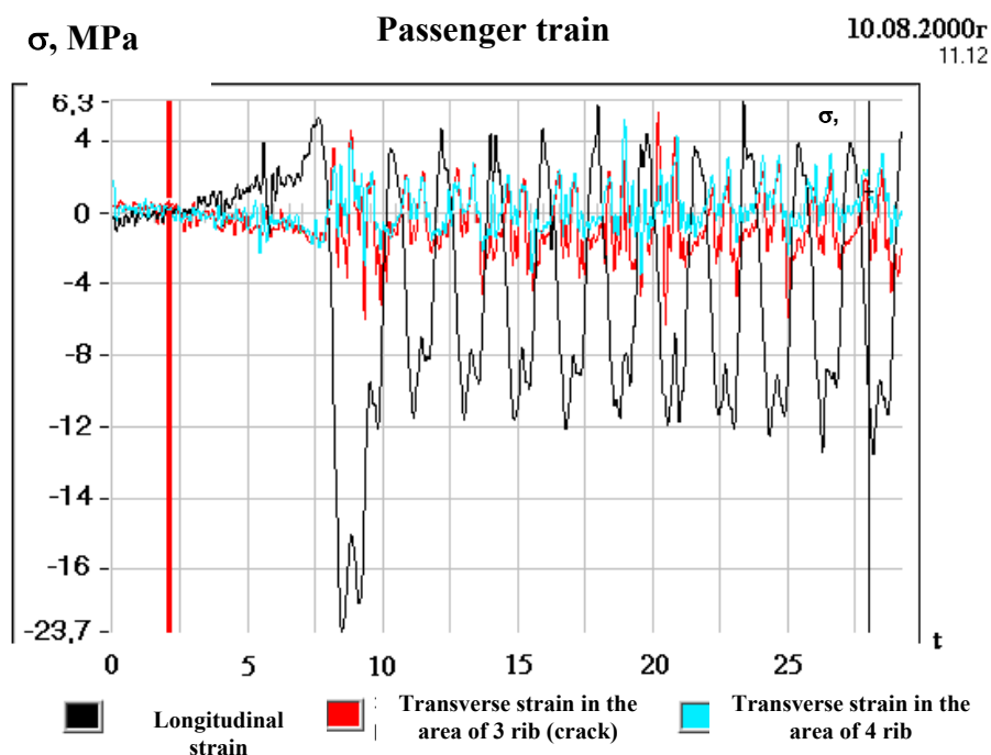
Fig.2. Strain measurement results for longitudinal girder
