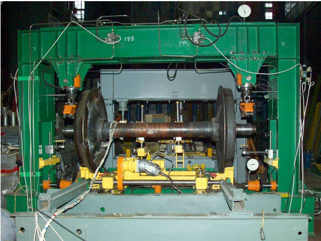
Fig.5. AE installation for wheelset pairs diagnostics
