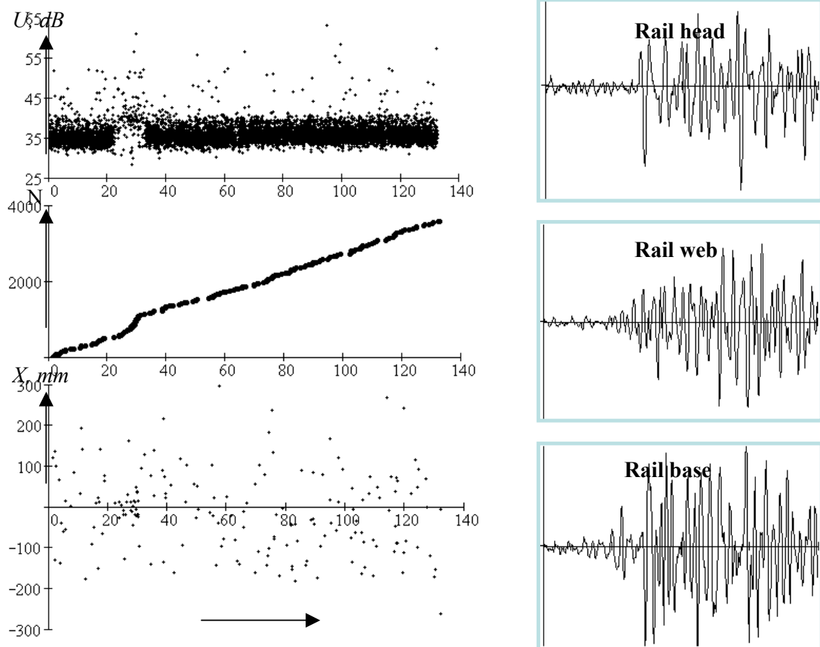
Fig.4. Characteristics of an acoustic emission sources detected and the form of acoustic emission impulses
