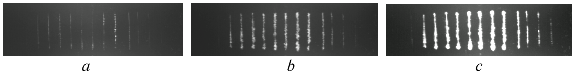
Fig.2. Defects indications revealed by fluorescent PT using the heating at several technological stages: a – conventional testing procedure (without heating): T_1 = 21^\circ\text{C} ; b - preliminary heating of test panel before penetrant application: T_2 = 49^\circ\text{C} ; c - combined heating of the panel at stages of penetrant and developer application T_2 = 49^\circ\text{C} , T_3 = 45^\circ\text{C} .
