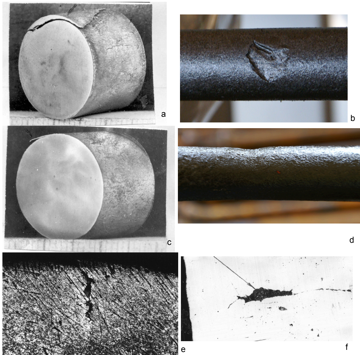
Fig.4. Microsection metallograhic specimens of some defects in the pump rods Ø19 mm: a - steelmaking defect - scab, b- mechanical impact defect - indent, c - rolling defect fold , d - shrinkage cavity, e - hair seams, f - slag inclusion
