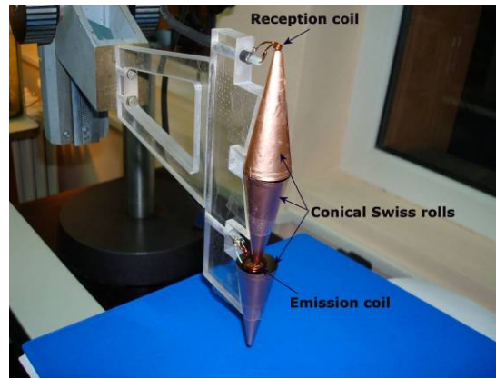
Figure 7. Electromagnetic transducer using conical Swiss roll
