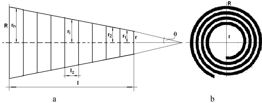
Figure 2. Conical Swiss roll: a) cross section; b) transversal view
