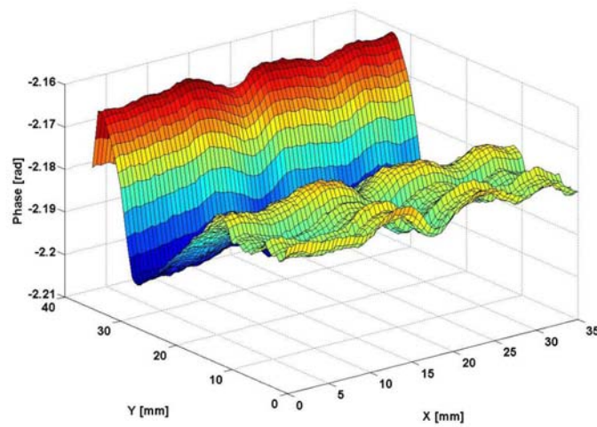
Figure 13. Signal delivered at the scanning of the sample with deformed cells by impact a) amplitude; b) phase
