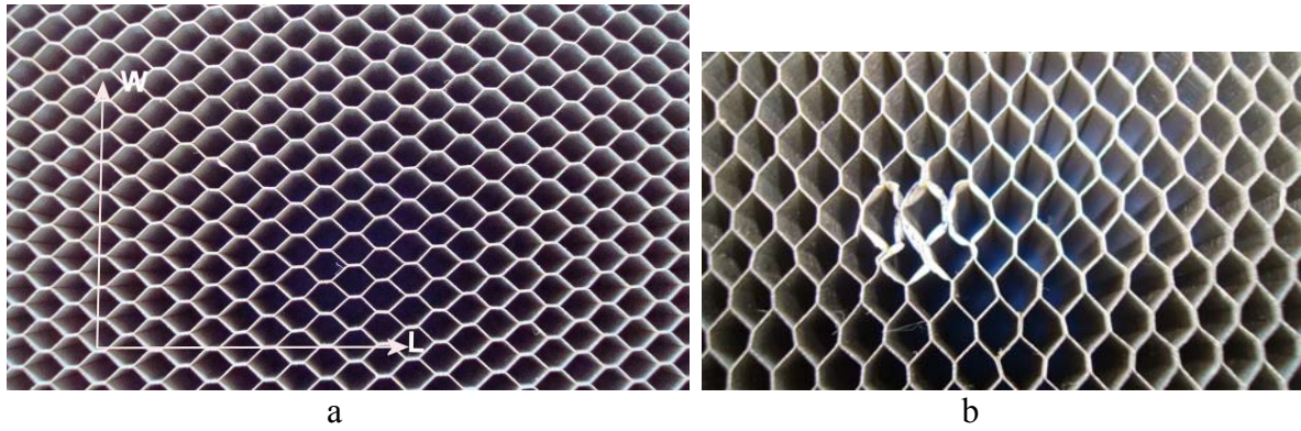
Figure 11. Honeycomb core AlMg with 1/6" cell's dimension a) reference sample; b) sample with cells deformed by impact
