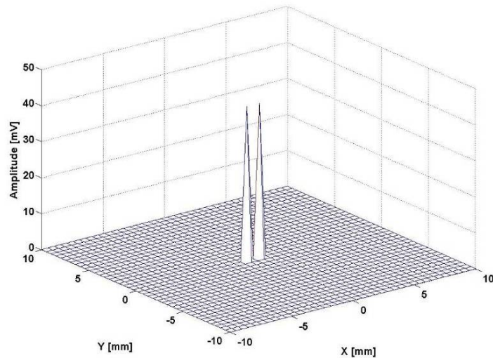
Figure 10. The response of the equipment at the scanning of region with two scatters
