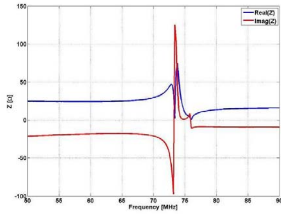
Figure 5. The dependency of impedance of a slab from conical Swiss roll by frequency
