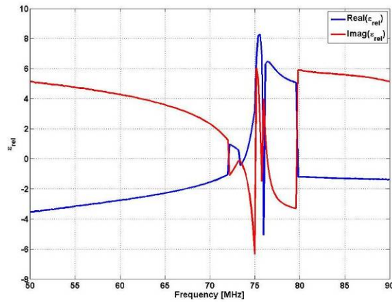
Figure 6. The dependency of electromagnetic parameters of a conical Swiss roll by frequency: a) relative magnetic permeability; b) relative dielectric permittivity
