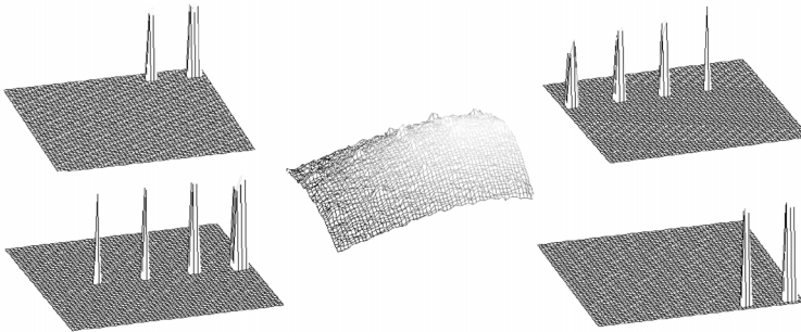
Fig. 2. Dynamic thermal tomography of a 1 mm-thick graphite epoxy sample (defects of different size at different depth, in centre – 'best' source image)
