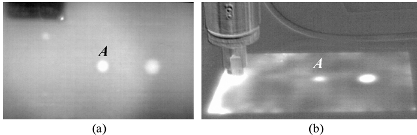
Fig. 1. Comparison between optical (flash tube 3 kJ) and ultrasonic stimulation (22 kHz) of a 1 mm-thick graphite epoxy composite:
