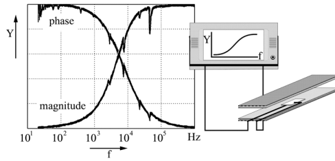
Fig. 1. Principal arrangement for impedance spectroscopy and spectrogram
