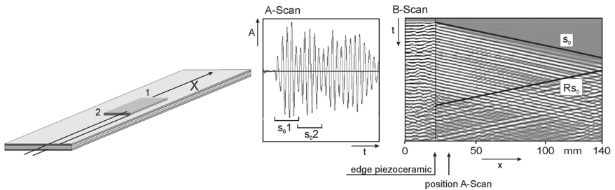
Fig. 2. Lamb-waves generated by integrated piezopatch: arrangement, A-scan, B-scan
