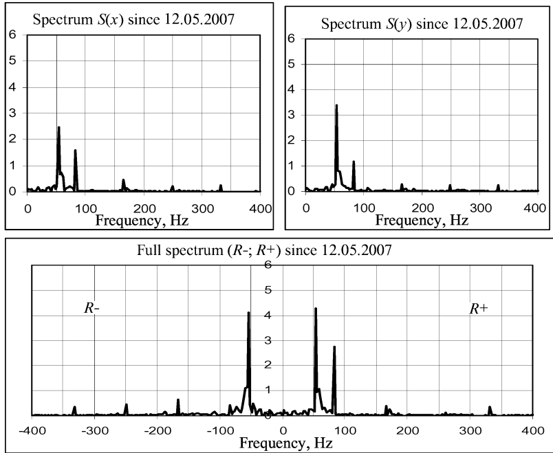
Fig. 2. Spectrums of horizontal S(x) and vertical S(y) relative vibrations of centrifugal force-pump field support (top) and corresponding full spectrum (bottom) one day before machine emergency stoppage
