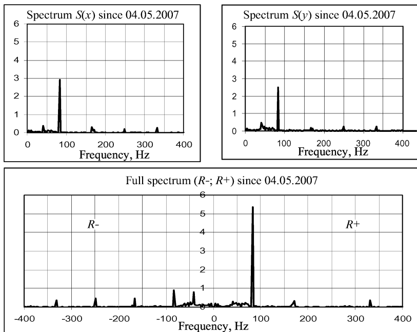
Fig. 1. Spectrums of horizontal S(x) and vertical S(y) relative vibrations of centrifugal force-pump field support (top) and corresponding full spectrum (bottom) seven days before machine emergency stoppage
