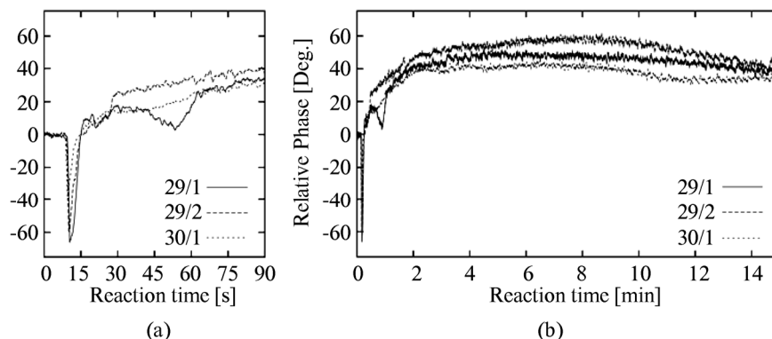
Fig. 1. Phase variation of the plate wave during foaming: start (a) and full time scale of the reaction (b)
